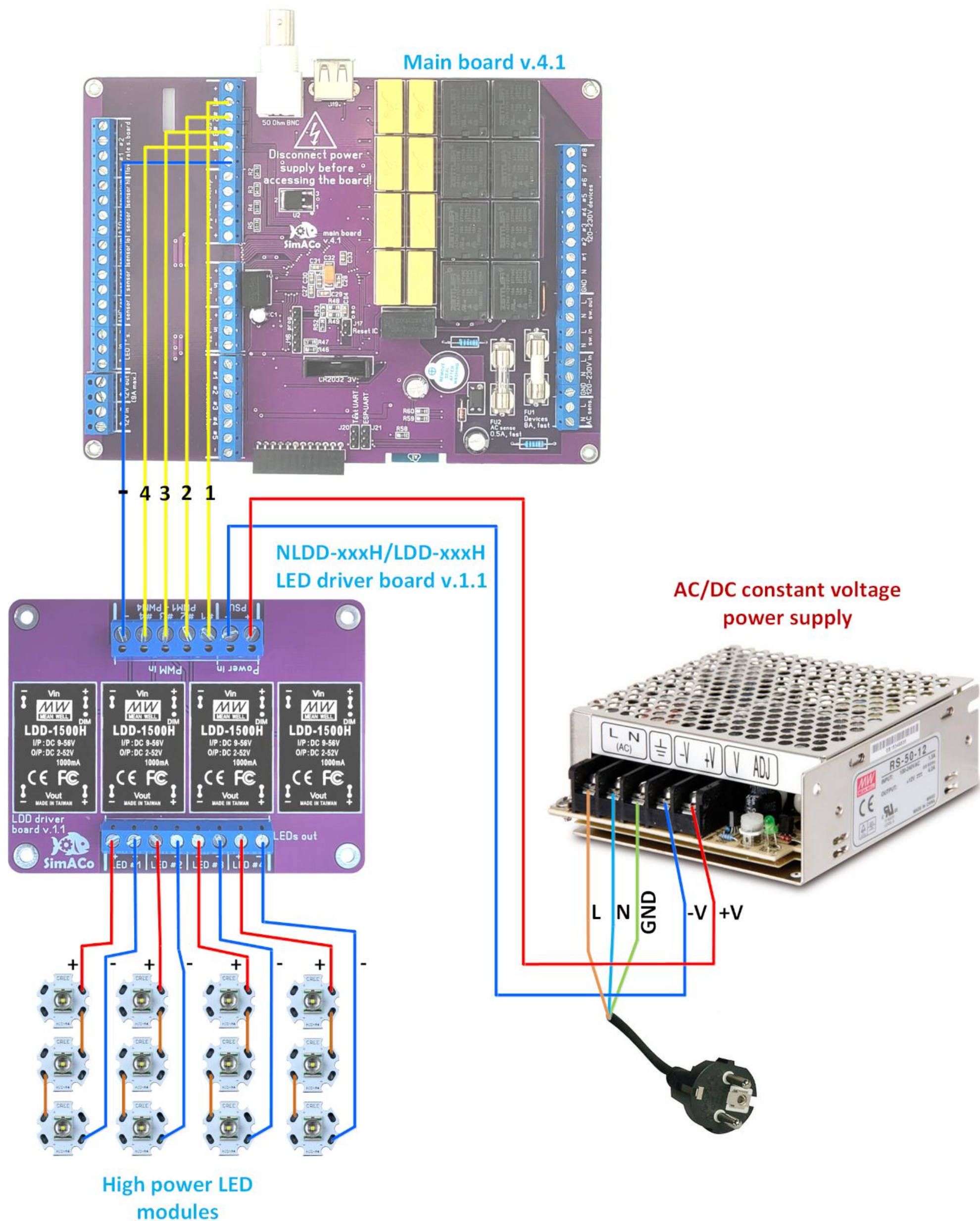
(N)LDD-H driver board v.1.1 connection diagram
